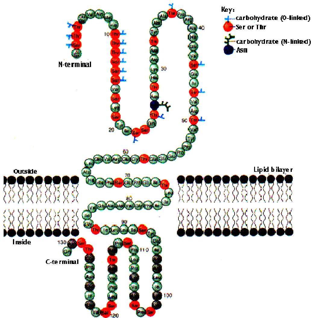
Fig.3.7. Primary structure of glycophorin A
