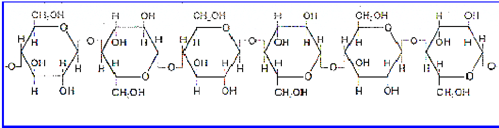
Fig.3.3d. Structure of Cellulose
