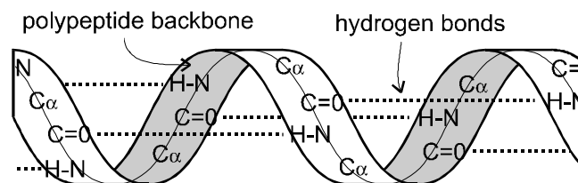
Fig.3.6b. The \alpha -helix Secondary Structure of Proteins
