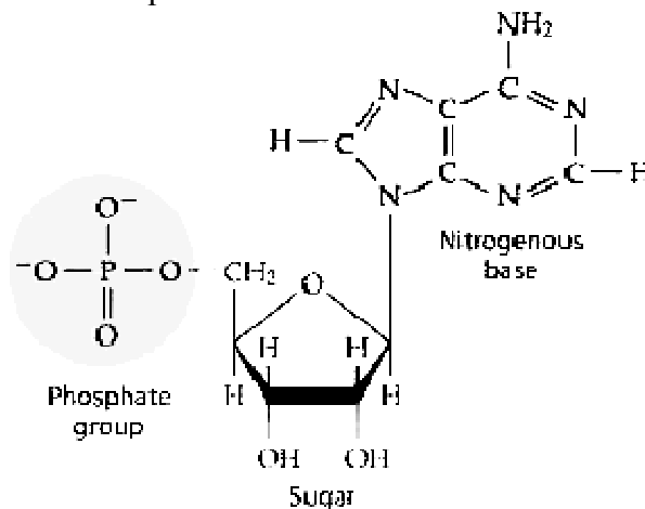
Fig.3.8b. Structure of a Nucleotide
