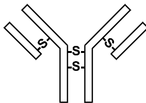
Fig.3.6e. Immunoglobulins
