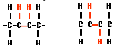
Fig.3.4d. Cis- and Trans- Configurations
