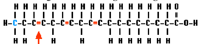
Fig.3.4c. Linolenic Acid, an omega-3 Fatty Acid
