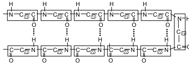
Fig.3.6c. The \beta -sheet Secondary Structure of Proteins
