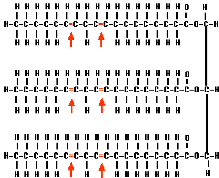
Fig.3.4b. Trilinolenin molecule
