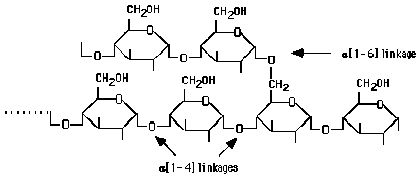
Fig.3.3c. Structure of glycogen
