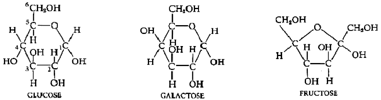
Fig.3.1. Examples of Monosaccharides
