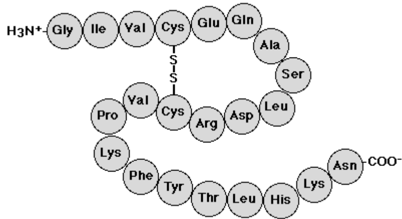
Fig.3.6a. Primary Structure of Polypeptide
