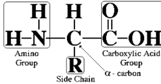
Fig.3.5a. Structure of Amino Acid
