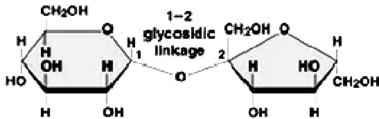
(b) Sucrose
