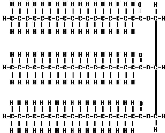
Fig.3.4a. Tristearin molecule
