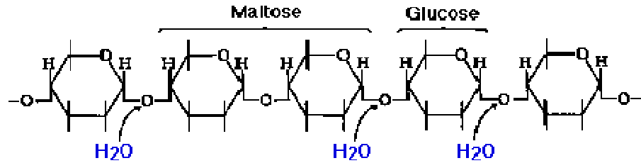
Fig.3.3b. Structure of amylopectin
